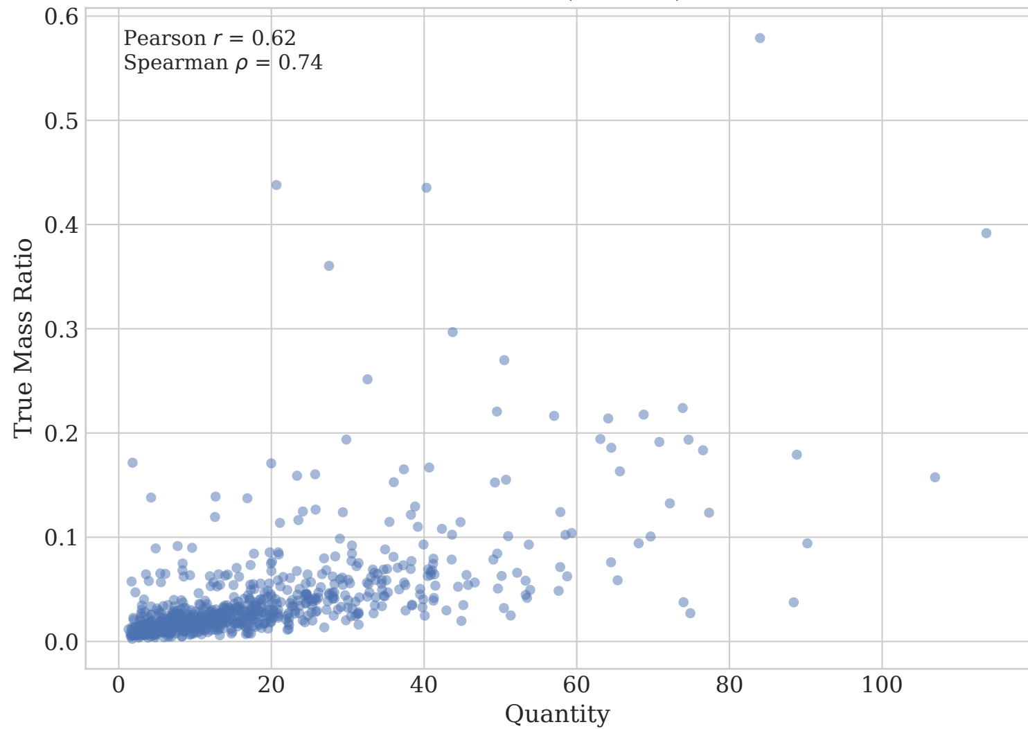
TNG300-1 (no noise)
