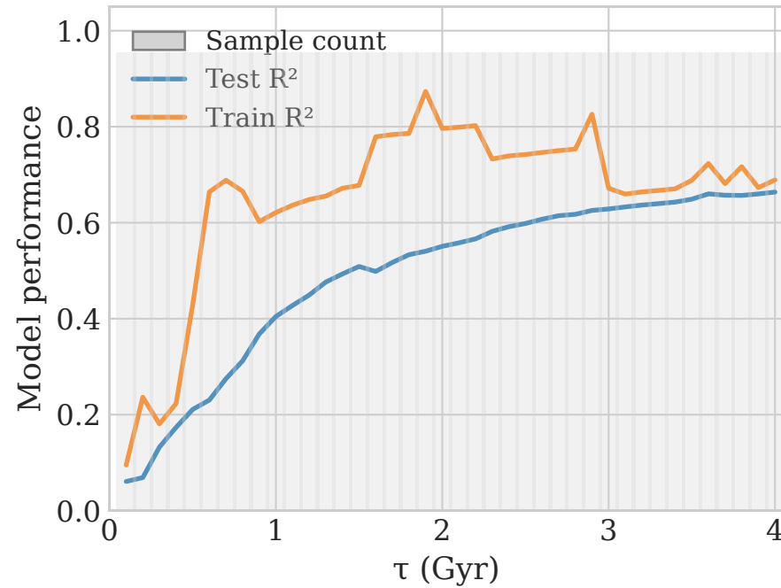
on past-merger score
