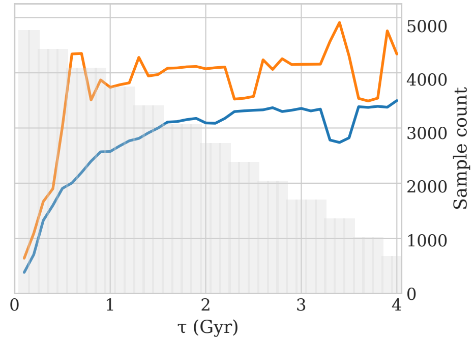
on full-merger score
