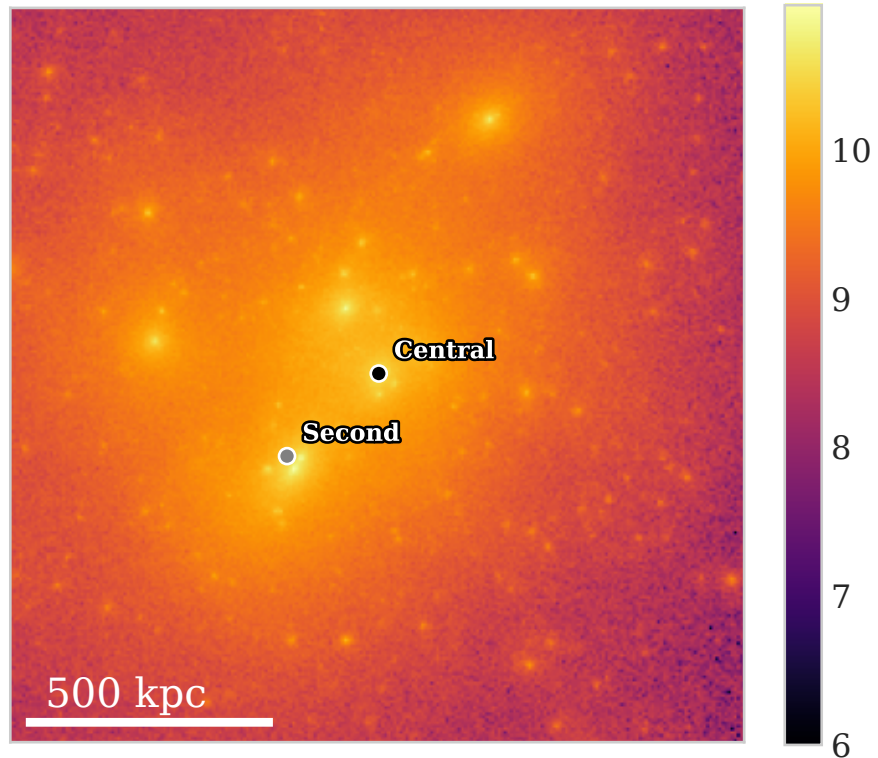
Surface Density ( \log M_{\odot} / \text{pixel} )
