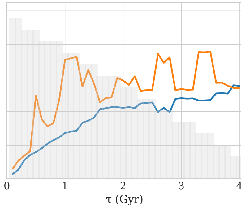
on future-merger score
