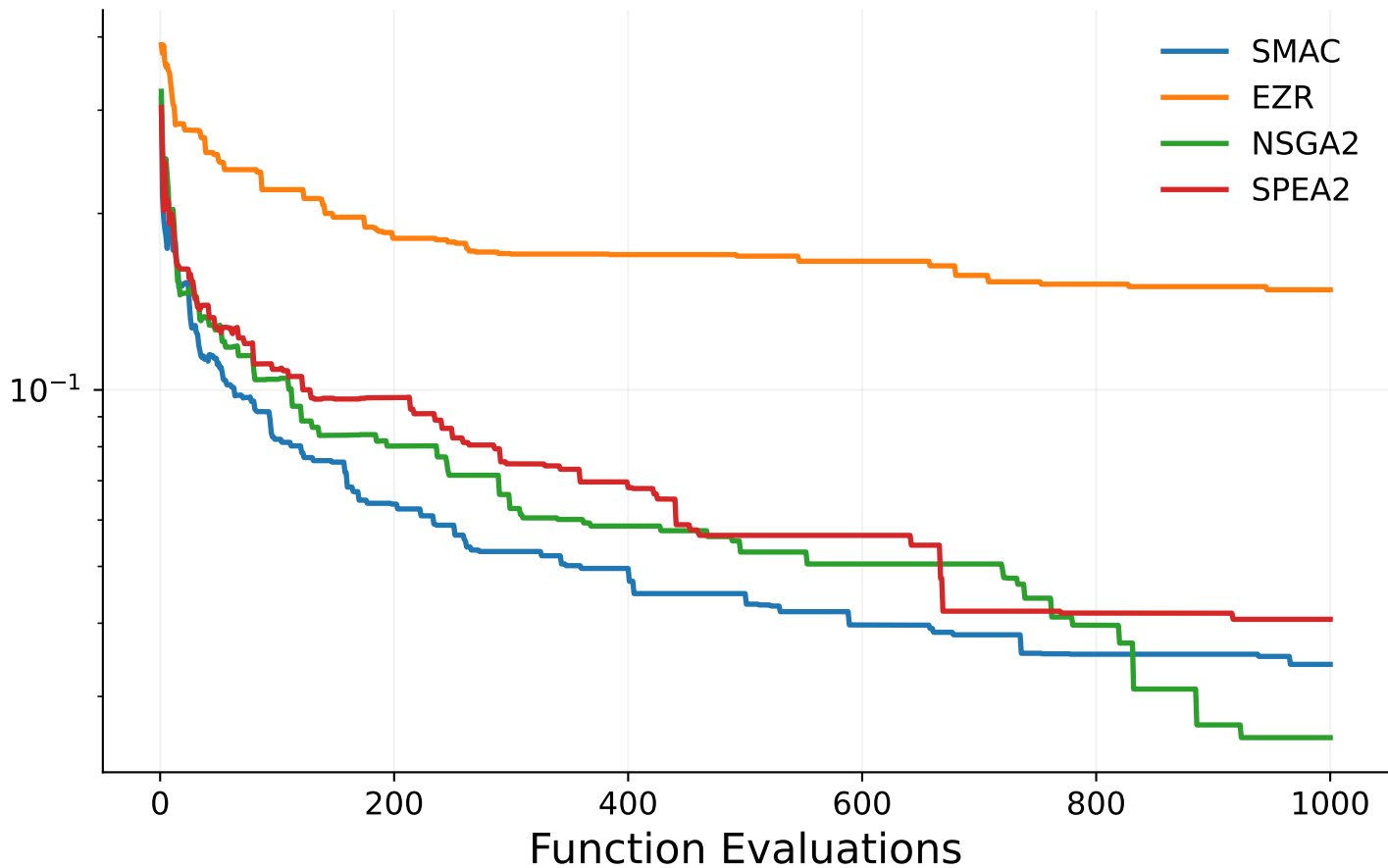
Dataset-level IQR (log scale)
