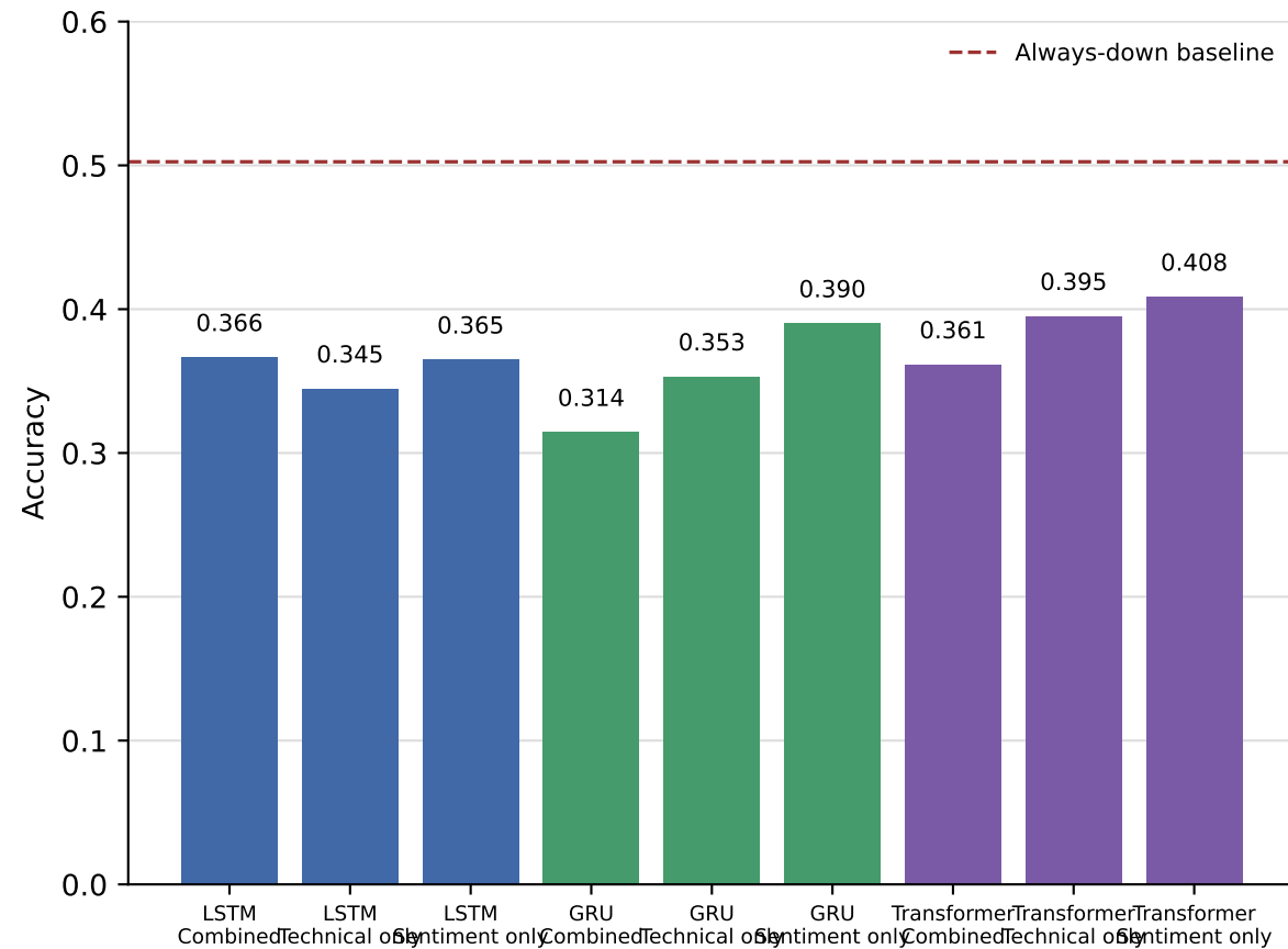
Test Directional Accuracy
