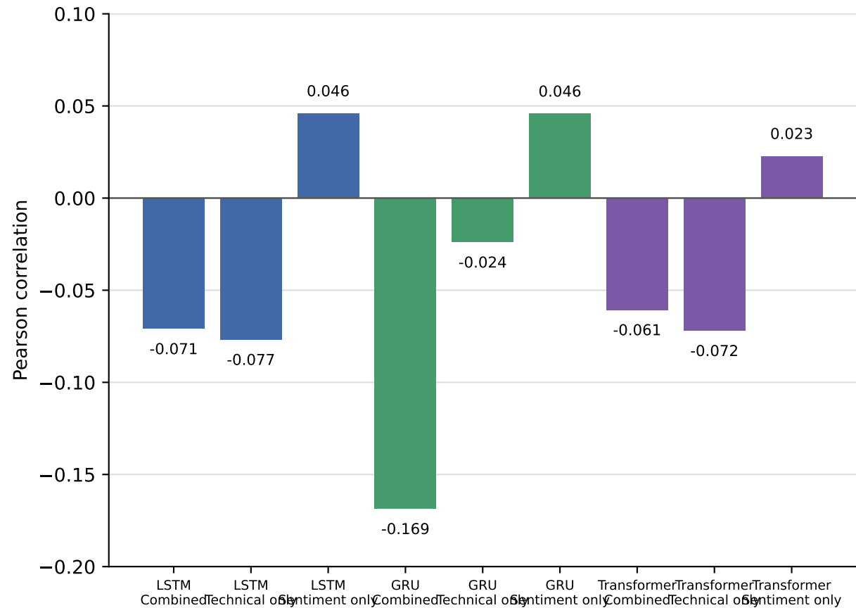
Test Return Correlation
