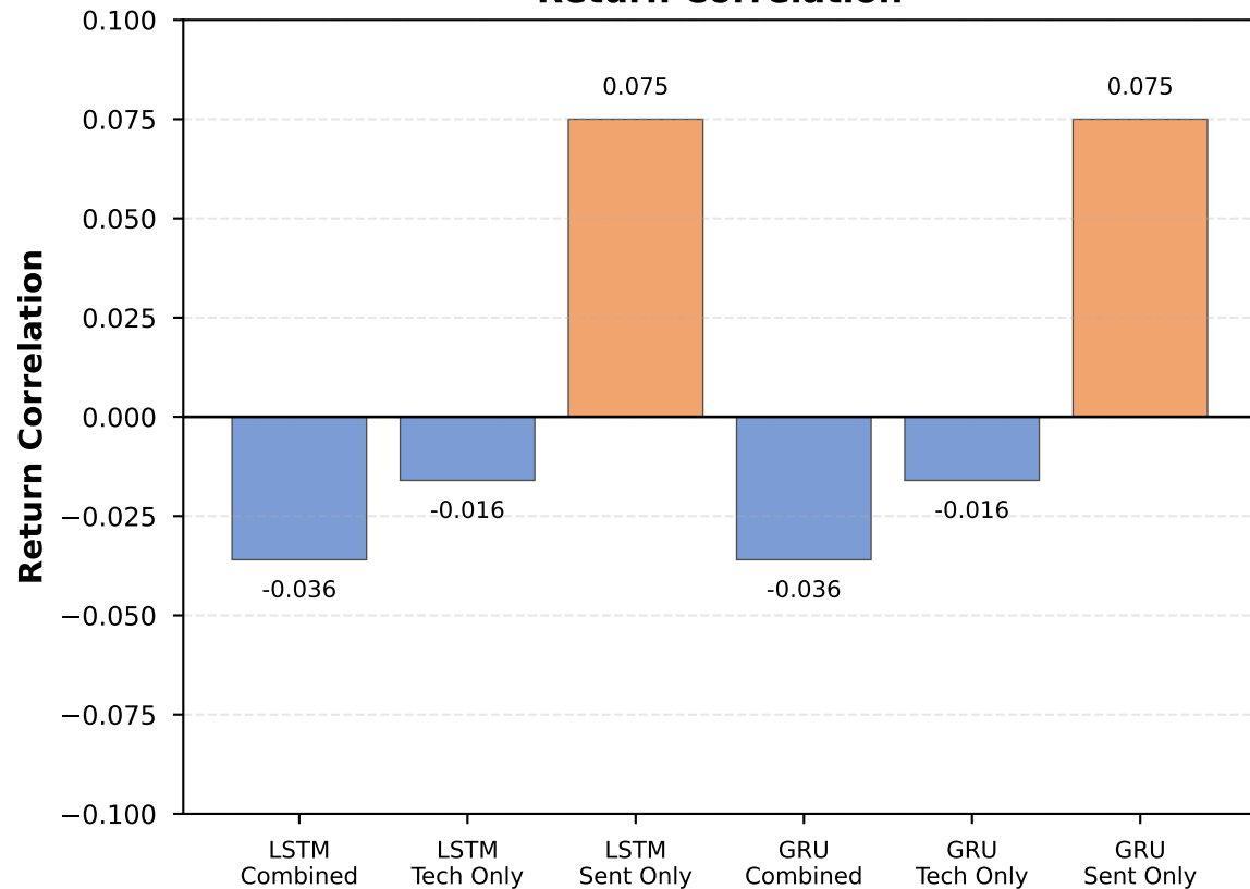
Return Correlation
