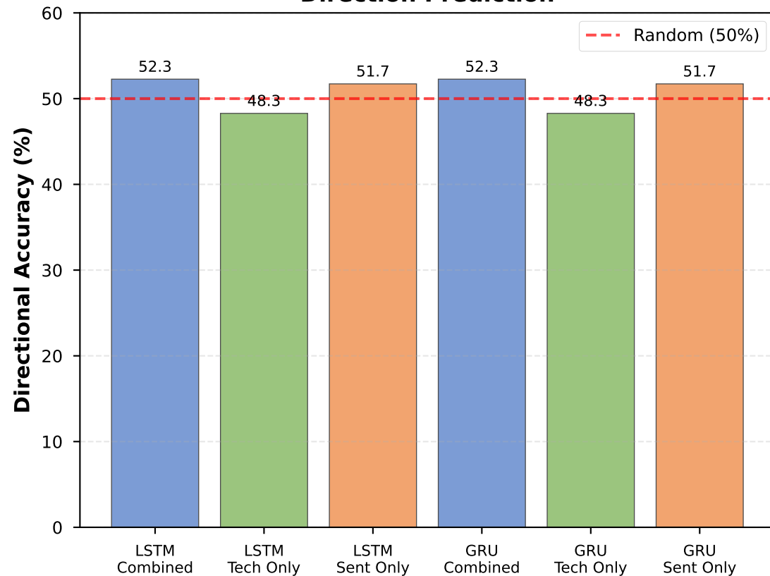
Direction Prediction
