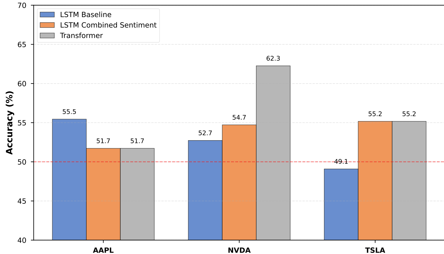
Per-Ticker Model Performance (2020-2022)
