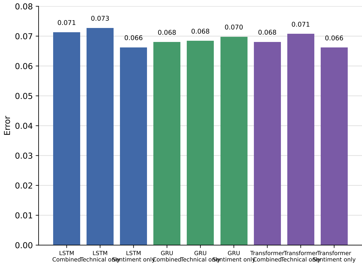
Test RMSE
