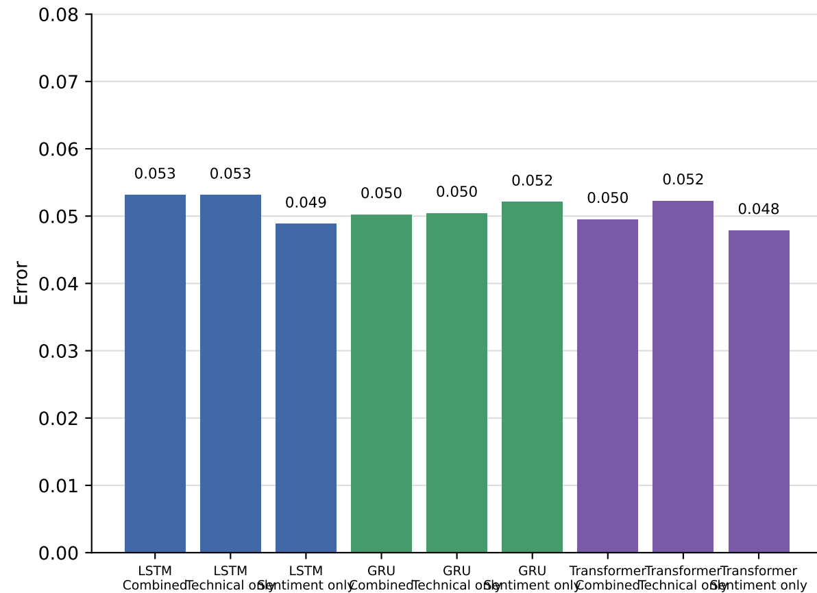
Test MAE
