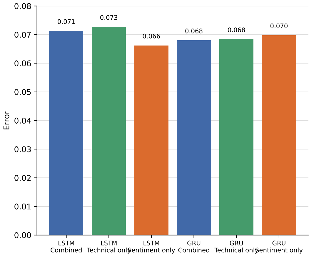
Test RMSE
