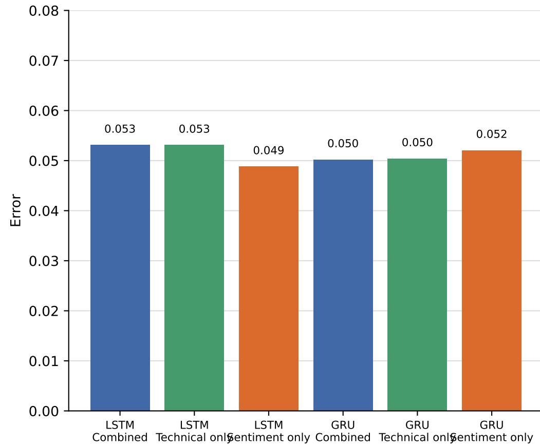
Test MAE
