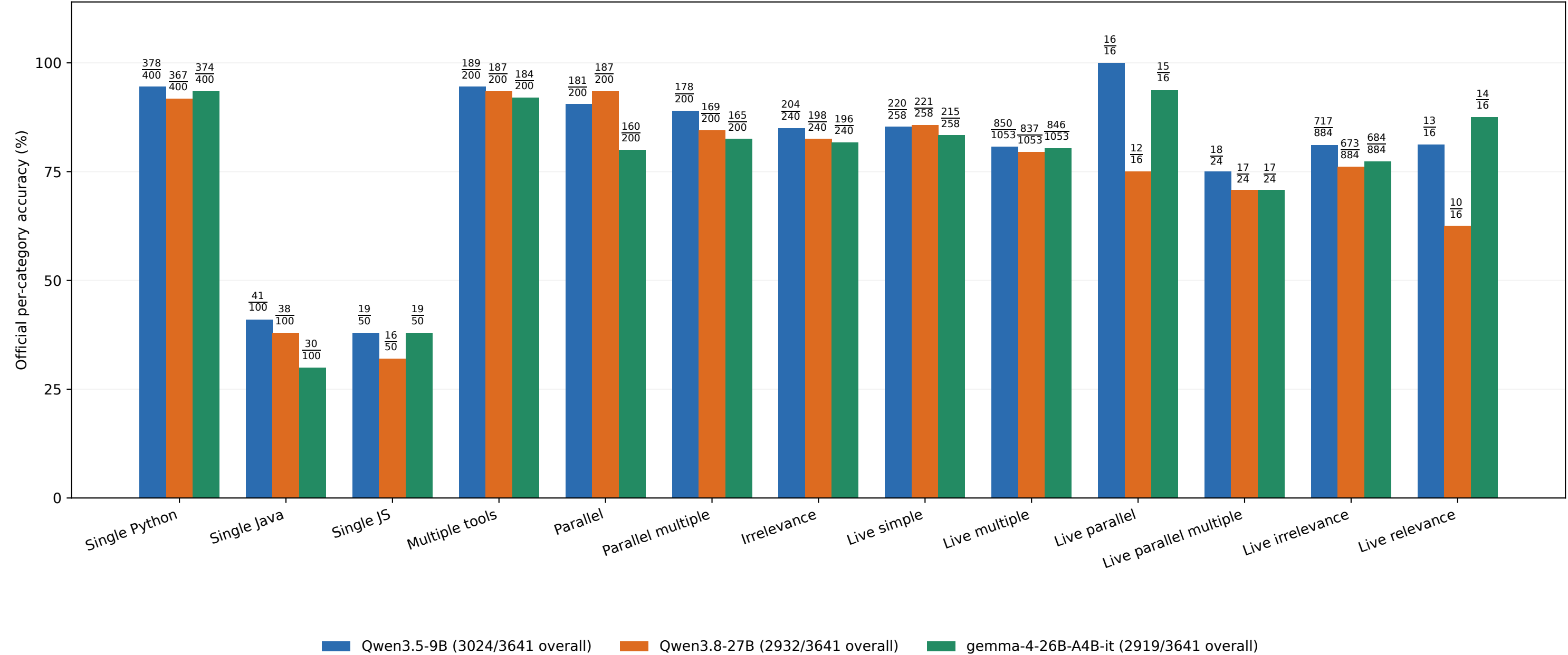
Tool-calling correctness on 3,641 fixed BFCL cases
