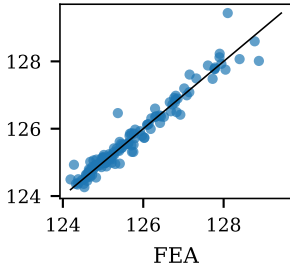
(b) max_vonMises_MPa
