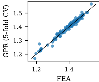
(a) mass_kg
