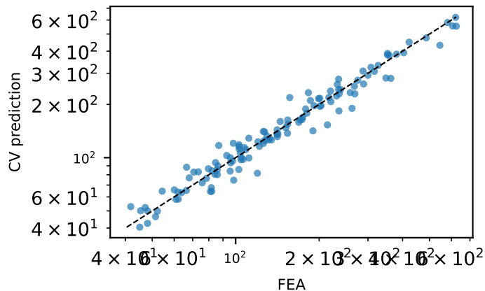
(c) von Mises, LC2 [MPa]
