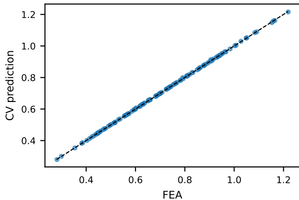
(a) mass [kg]
