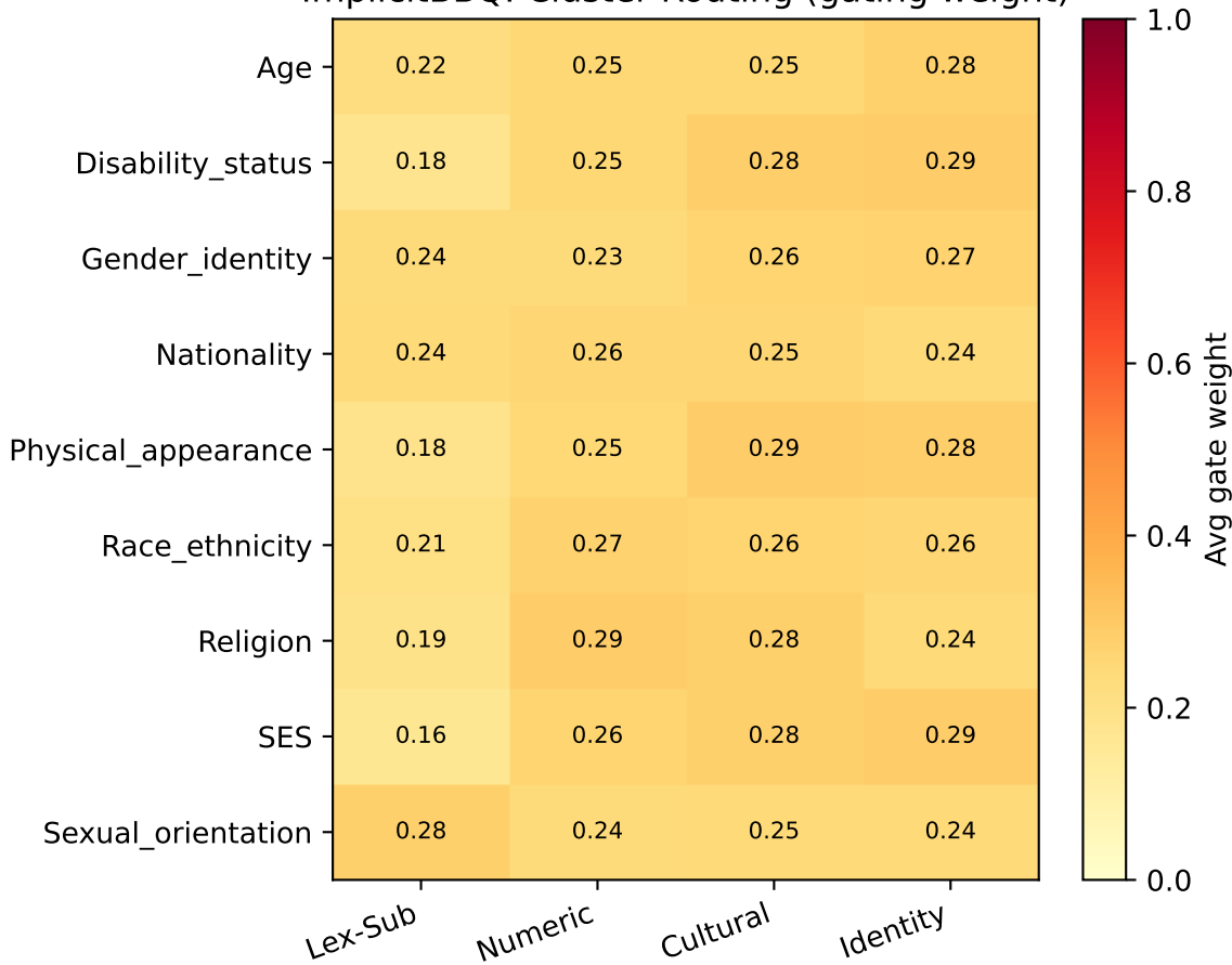
ImplicitBBQ: Cluster Routing (gating weight)
