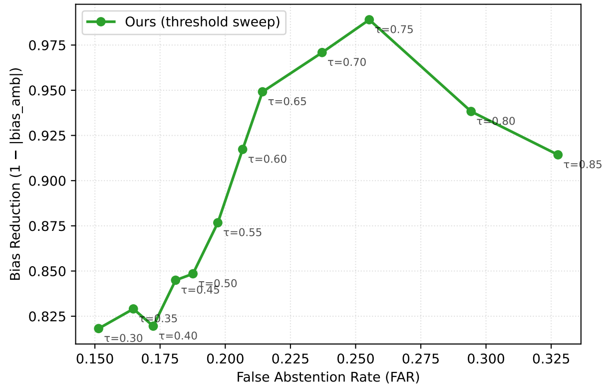
Risk-Coverage Trade-off
