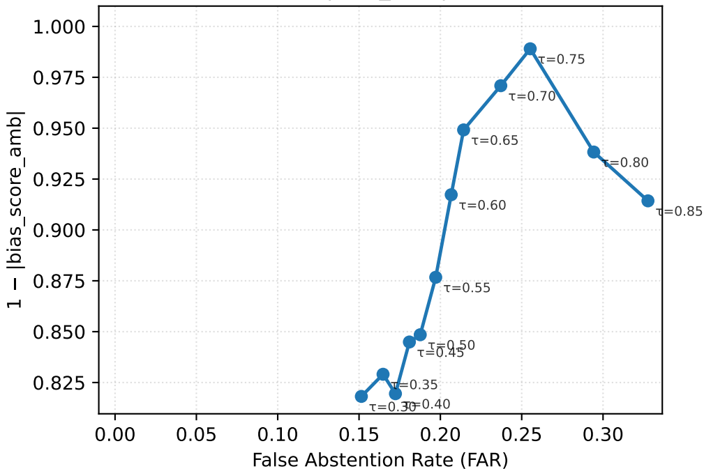
FAR vs 1 - |\text{bias\_amb}| trade-off
