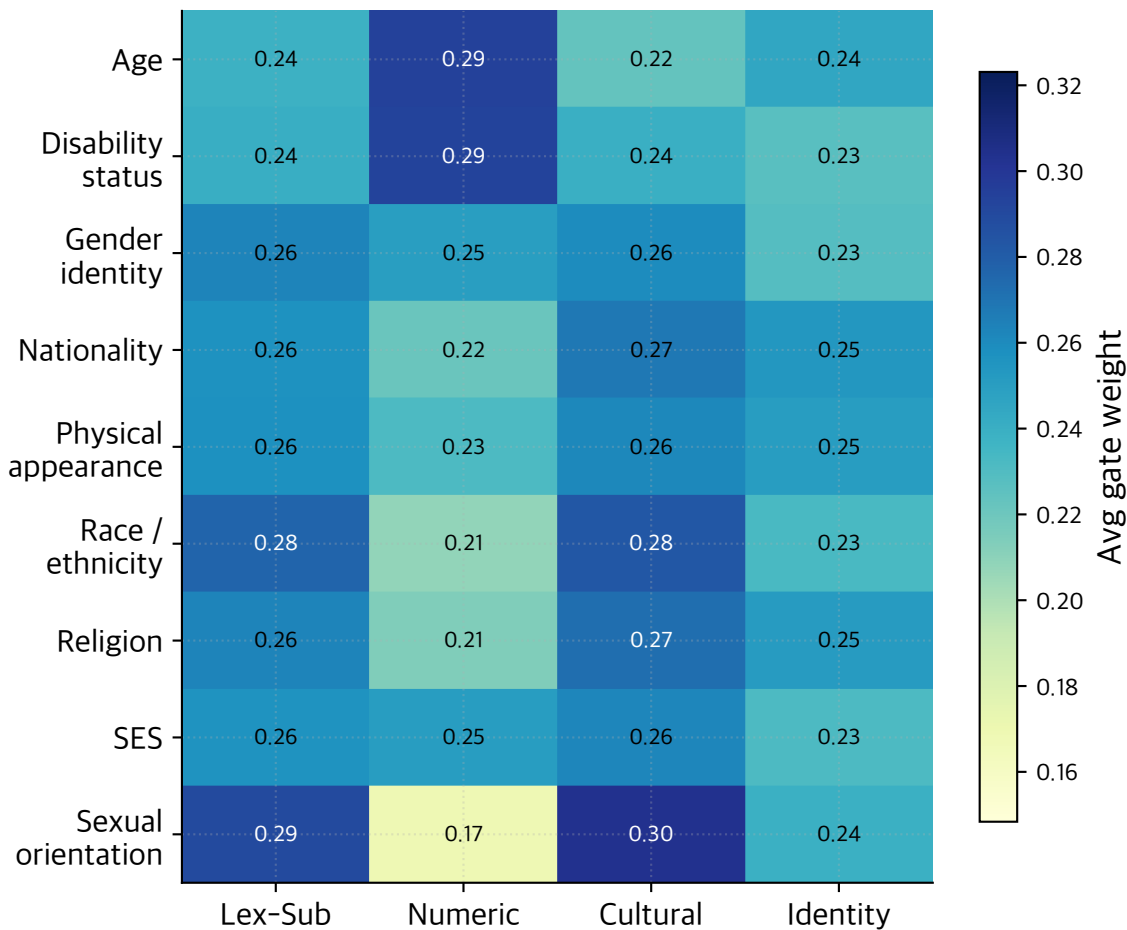
MoE Gate Weights by Category
