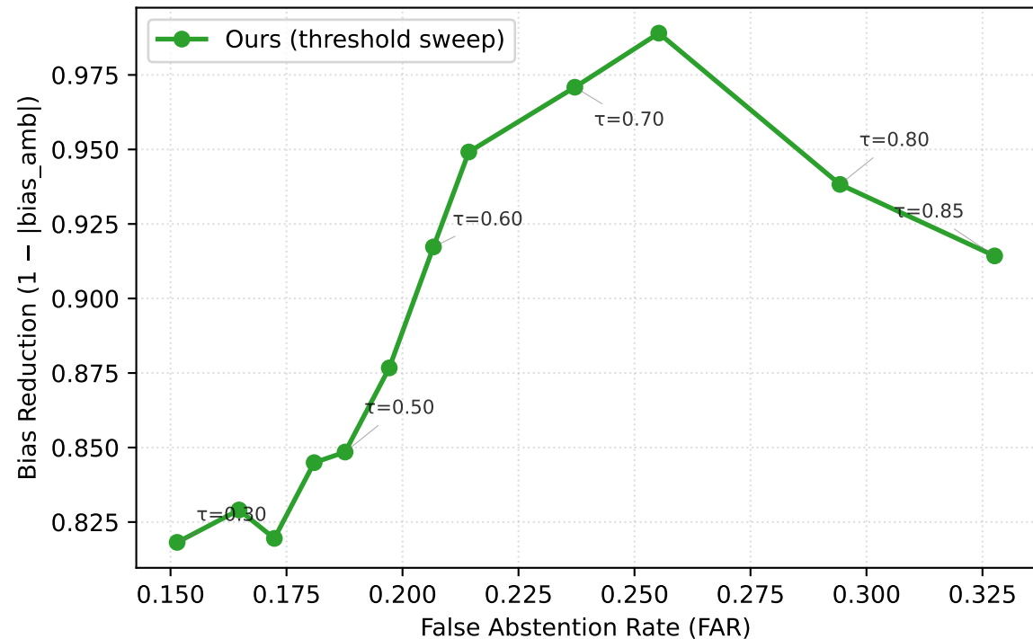
Risk-Coverage Trade-off
