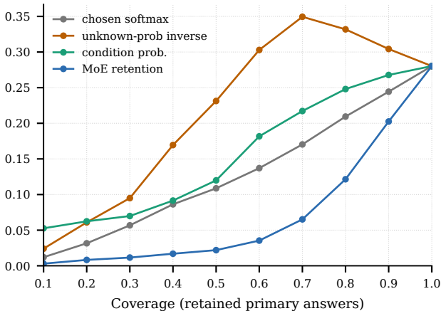
Selective risk
