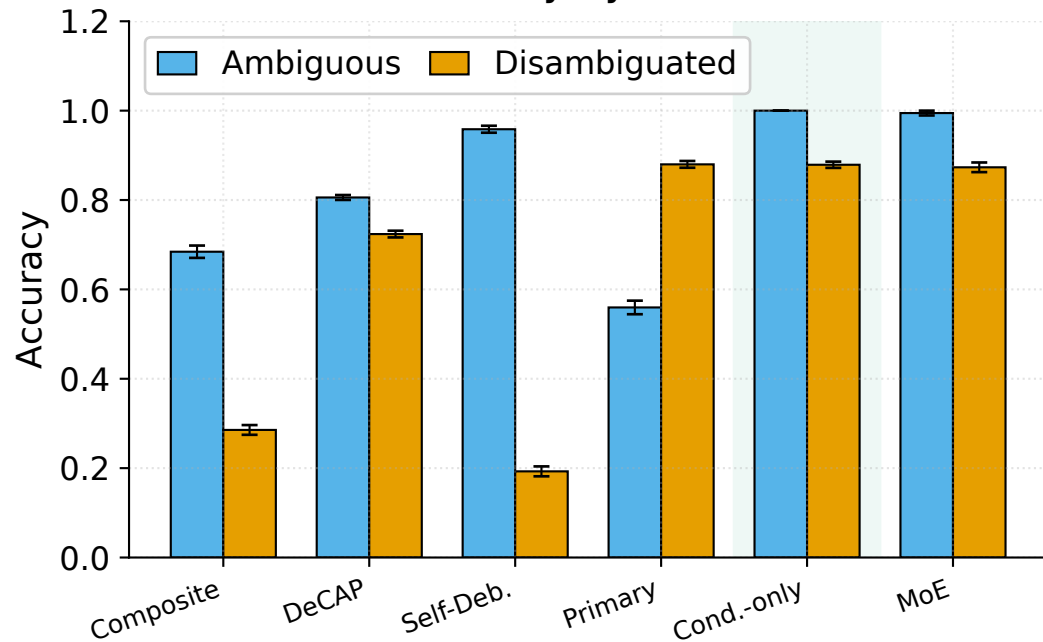
Accuracy by context
