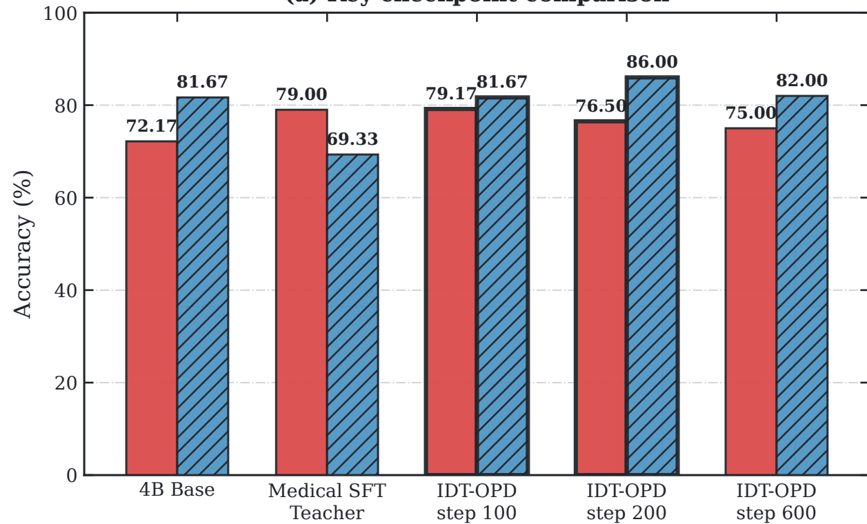
(a) Key checkpoint comparison
