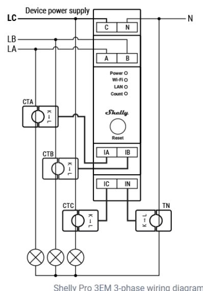
Shelly Pro 3EM 3-phase wiring diagram
