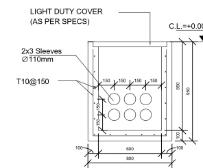
TYPICAL SECTION FOR ICT 1 : 20
