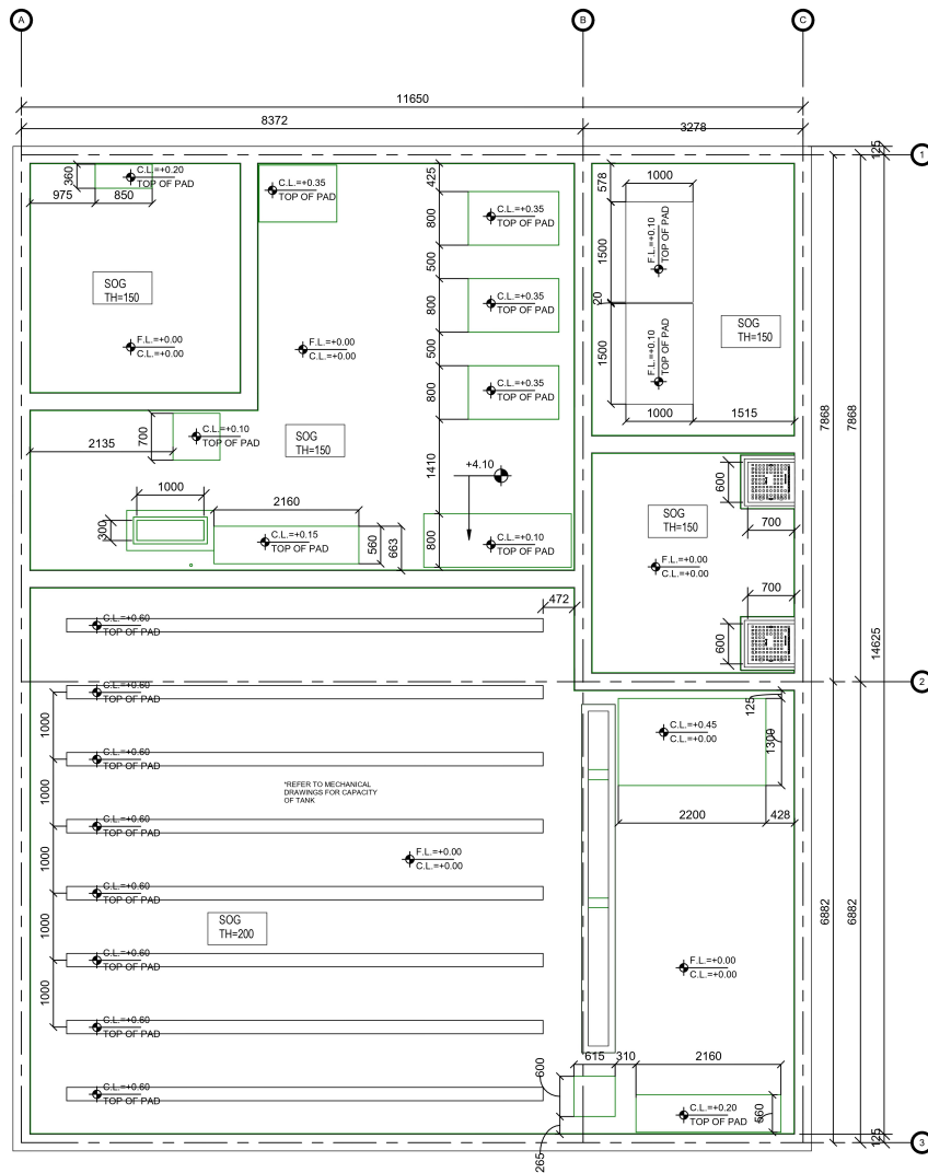
Concrete pad layout 1 : 50
