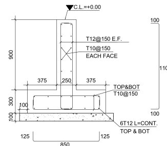
TYPICAL SECTION ON LF1 Sc.:1/25
