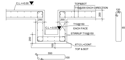
TYPICAL SECTION ON TRENCH AND SOG (Th=200) REINF DETAIL Sc.:1/25
