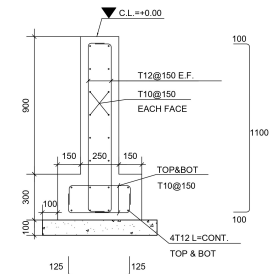
TYPICAL SECTION ON LF2 Sc.:1/25
