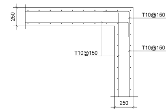
UNDERGROUND WALL CONNECTION - HZ REINF DISTRIBUTION AT CORNERS Sc.:1/25
