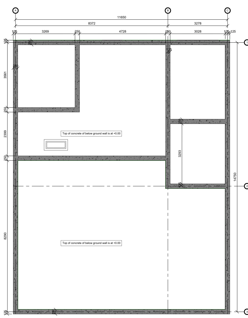
RC WALL BELOW GF FRAMING LAYOUT
