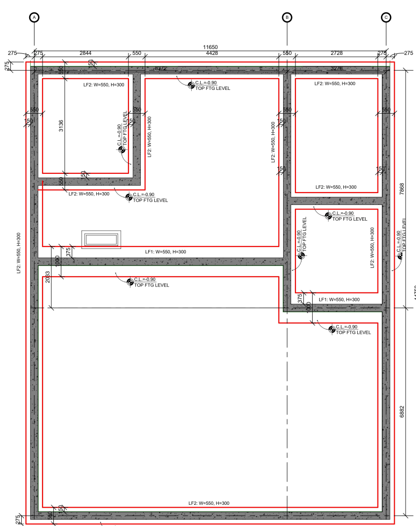
FOUNDATION FRAMING LAYOUT
