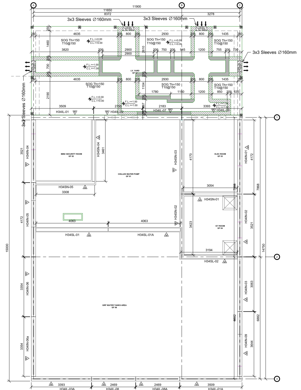
GROUND FLOOR PLAN -PC WALL PANEL LAYOUT 1 : 50
