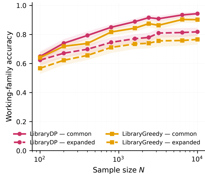
(a) Working-family accuracy
