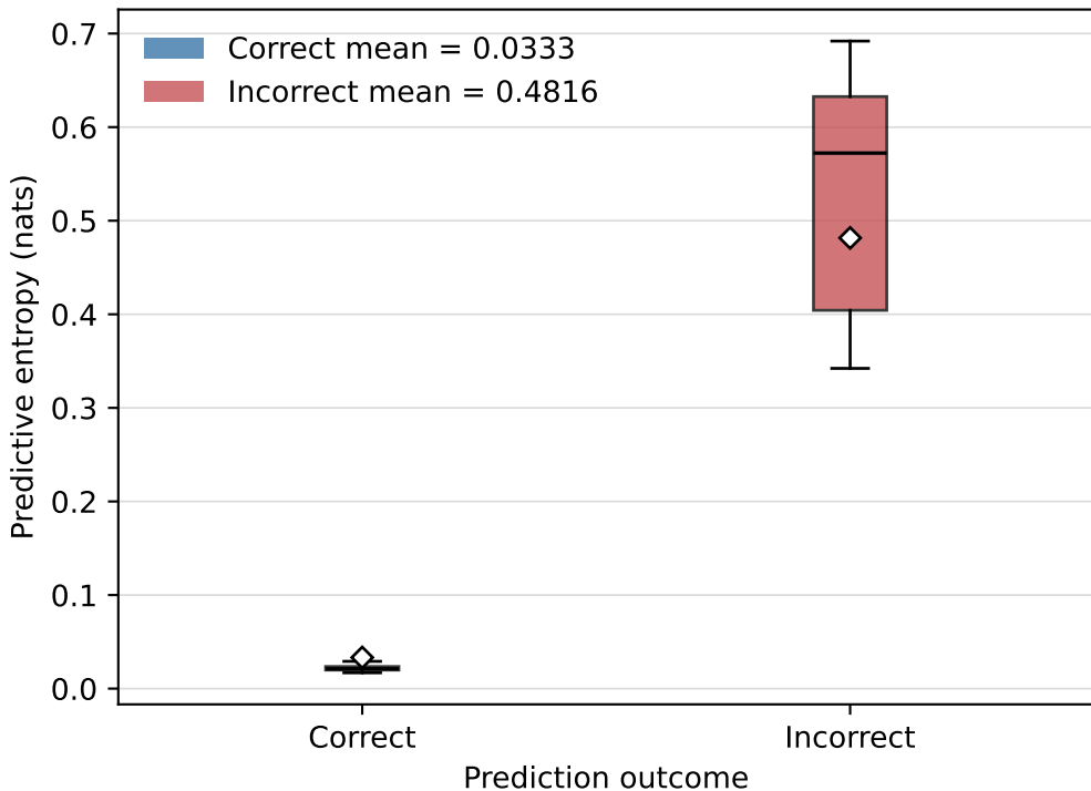
Predictive entropy by classification outcome
