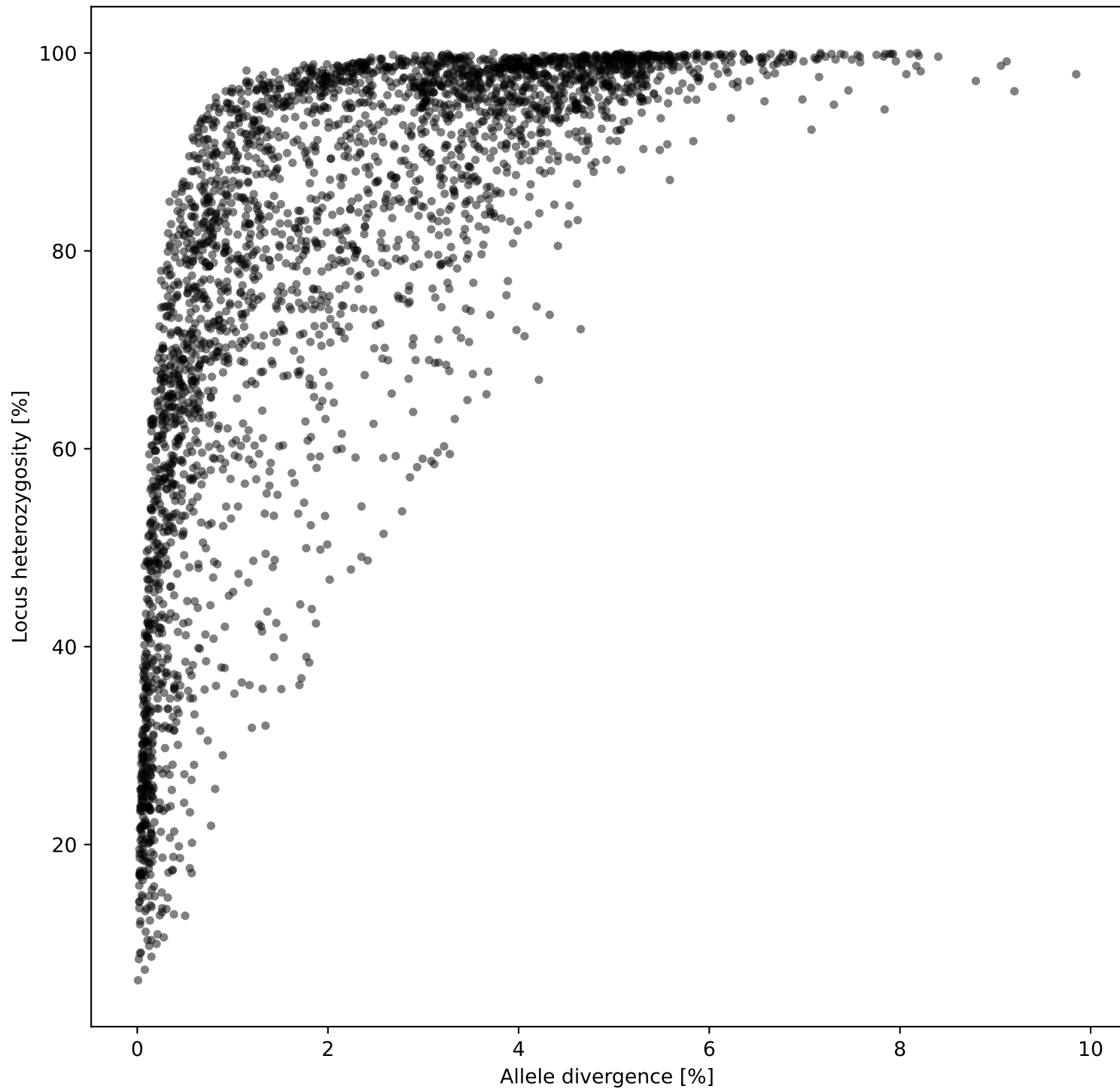
Locus heterozygosity vs allele divergence (combined)
