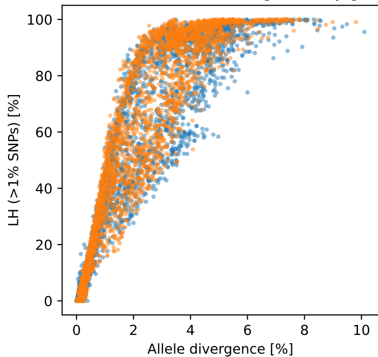
LH (>1% SNPs) vs allele divergence (by genome)
