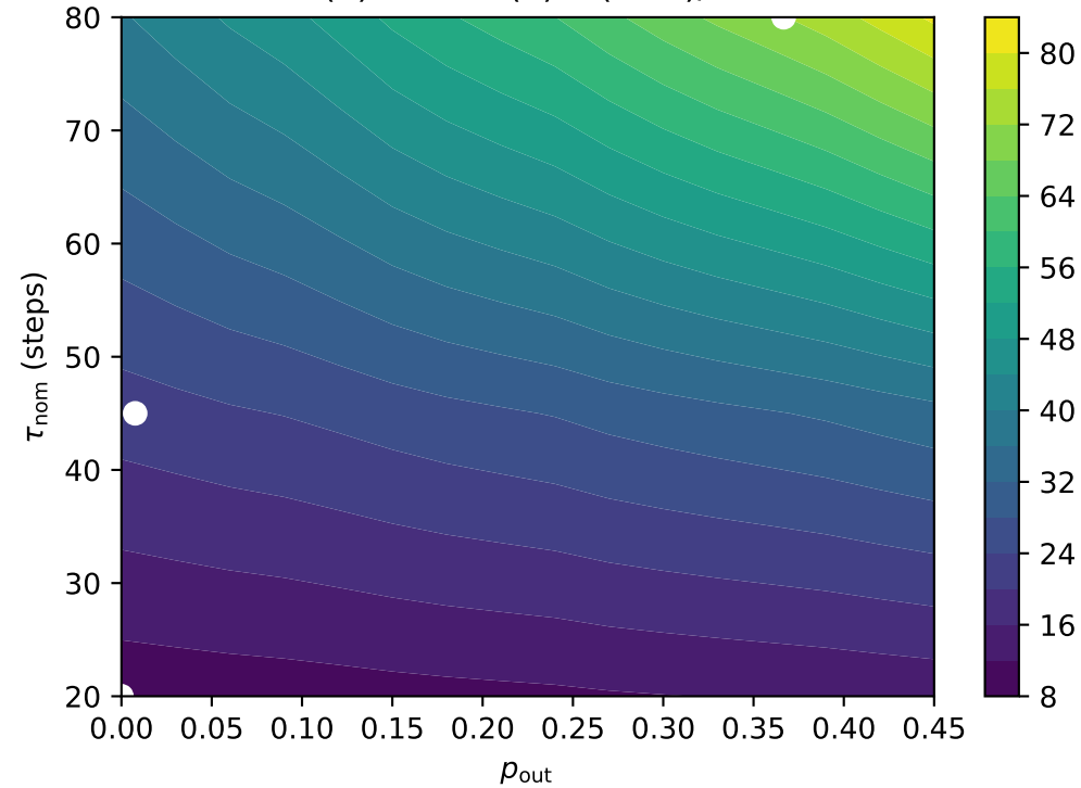
(a) Mean \kappa(\tau) = (\tau-1)/2
