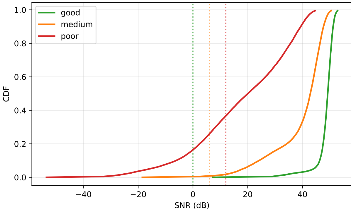
Empirical SNR CDF by link class (dotted: \gamma_{th} )
