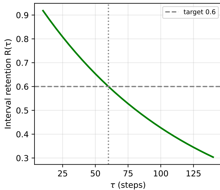
Staleness calibration curves
