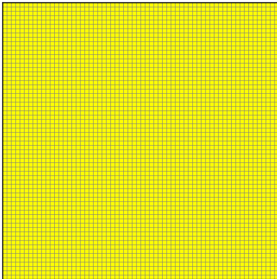
Aligned Spins
