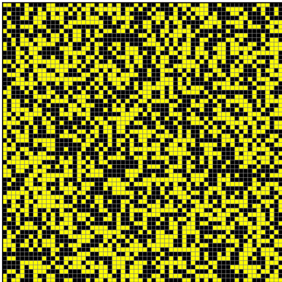
Random Spins
