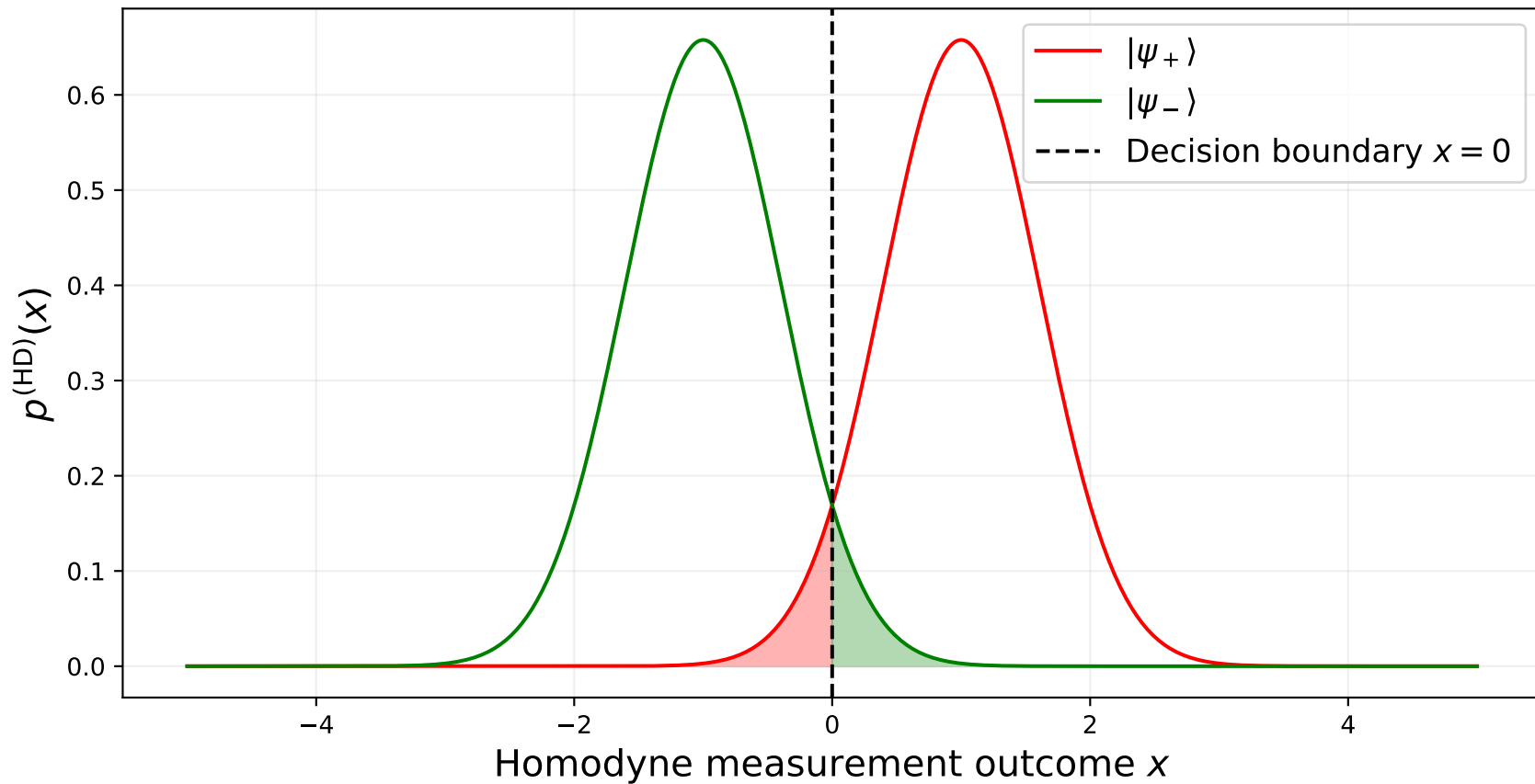
Homodyne distributions: \alpha = 0.5, r = 0.5
