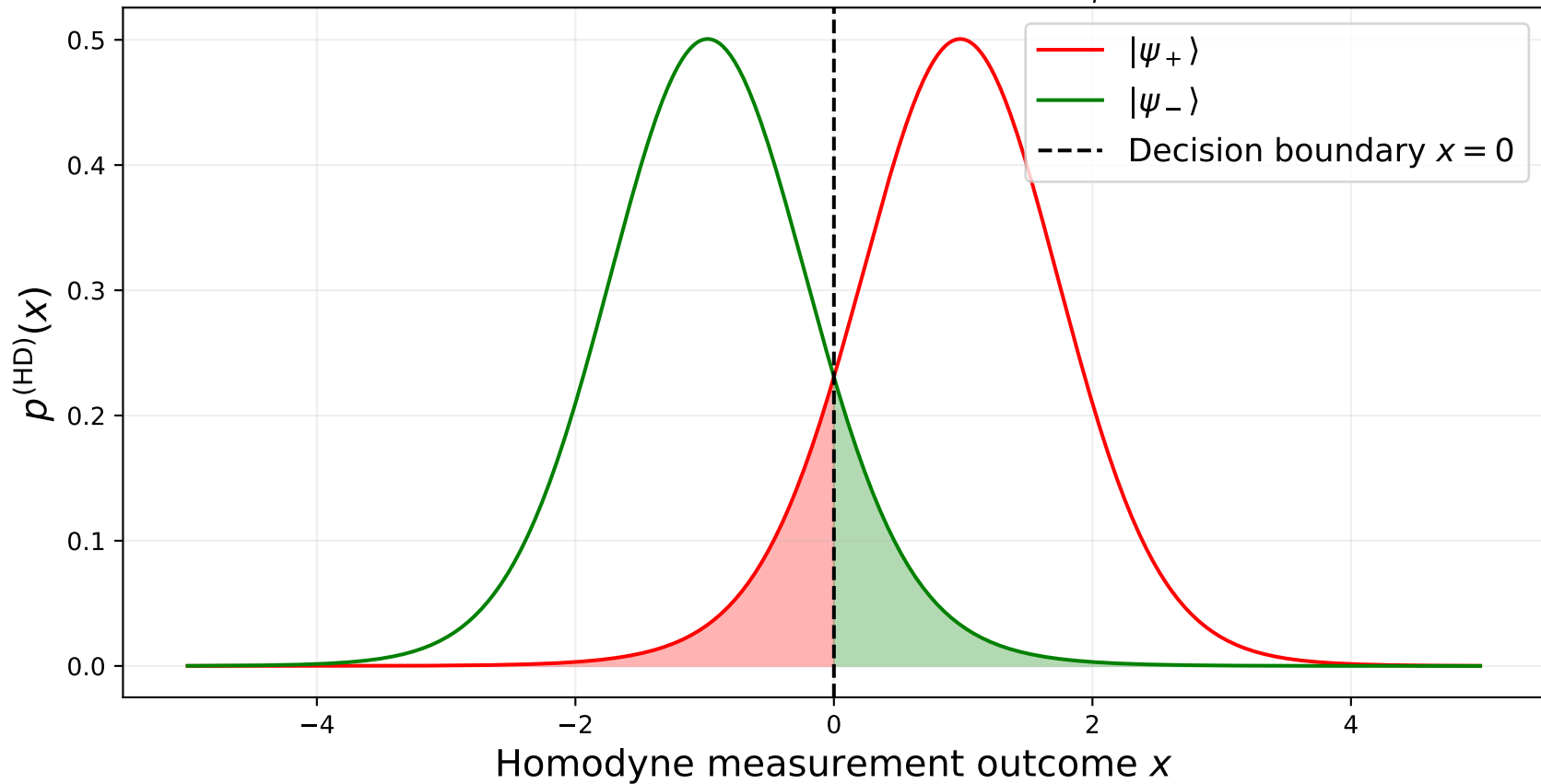
Homodyne distributions: \alpha = 0.5 , r = 0.5 , \sigma_\phi = 0.3 , \mu = 0.8
