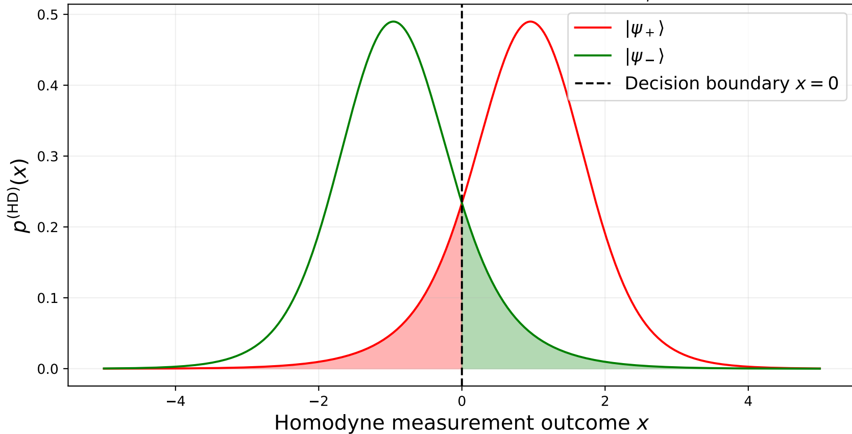
Homodyne distributions: \alpha = 0.5, r = 0.5, \sigma_\phi = 0.5
