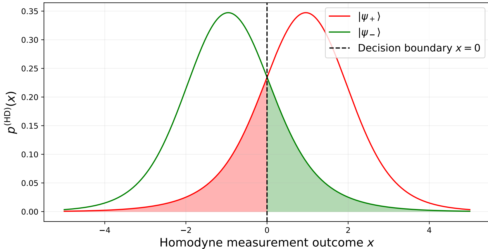
Homodyne distributions: \alpha = 0.5 , r = 0.5 , \sigma = 0.5 , \mu = 0.5
