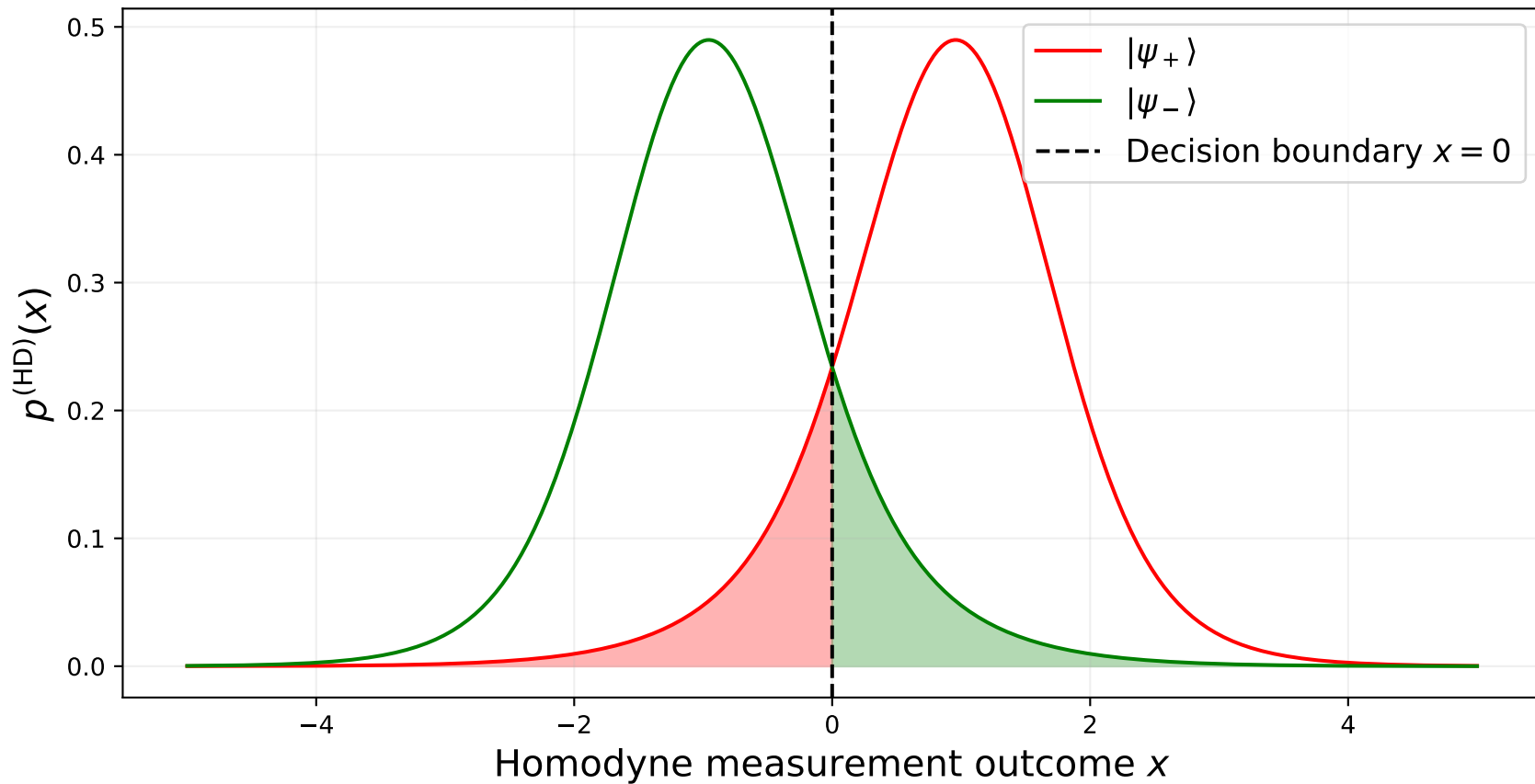
Homodyne distributions: \alpha = 0.5 , r = 0.5 , \sigma = 0.5
