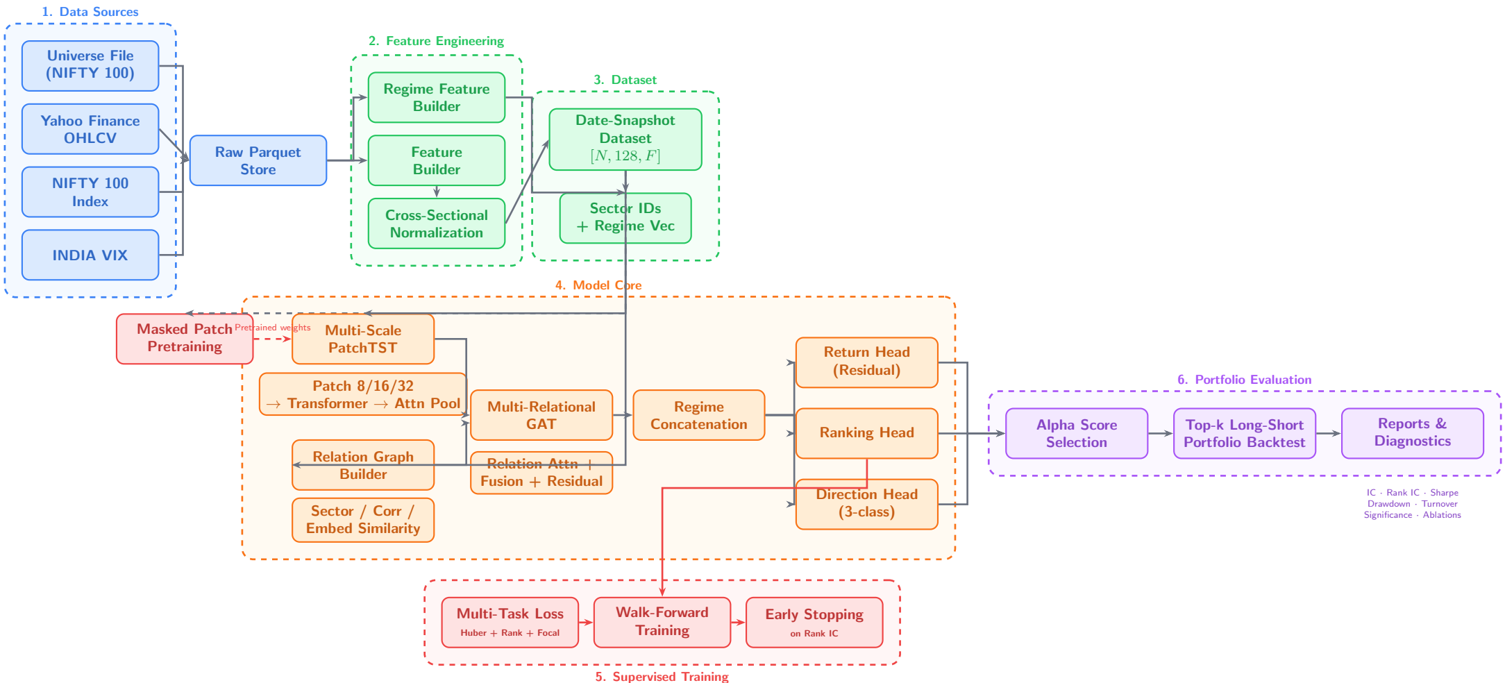
End-to-end architecture of the NIFTY 100 cross-sectional forecasting system. Daily stock, index, and VIX data are converted into cross-sectionally normalized feature tensors. A multi-scale PatchTST encoder generates stock embeddings refined via a multi-relational GAT. Regime-aware multi-task heads predict residual return, ranking score, and direction, evaluated in a walk-forward top-k long-short portfolio framework.
