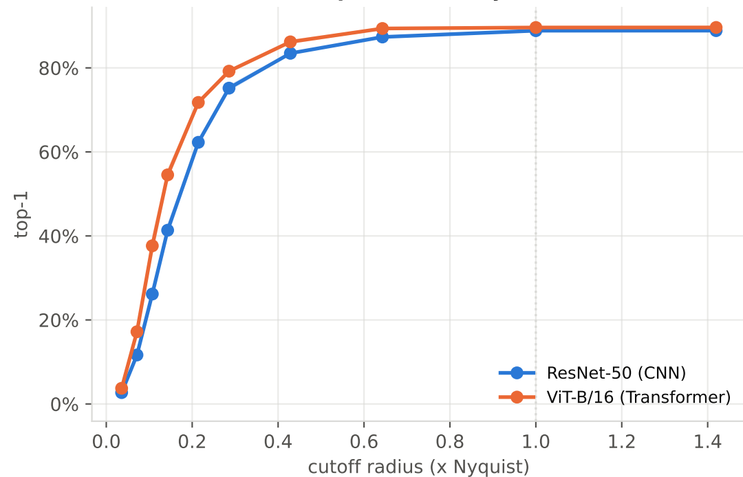
Ideal low-pass: accuracy vs cutoff
