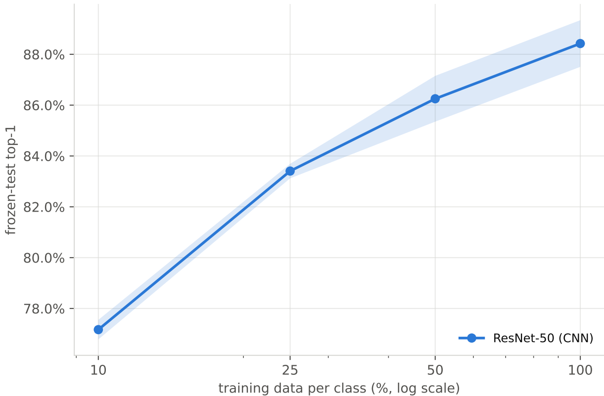
Data efficiency under a controlled transfer protocol
