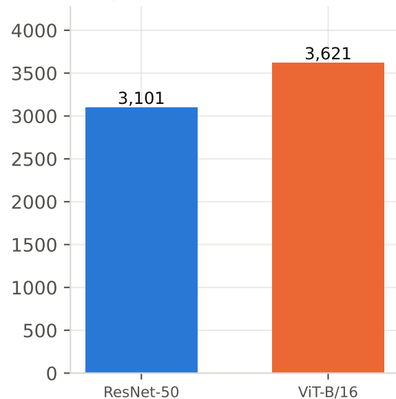
peak train VRAM (MB)
