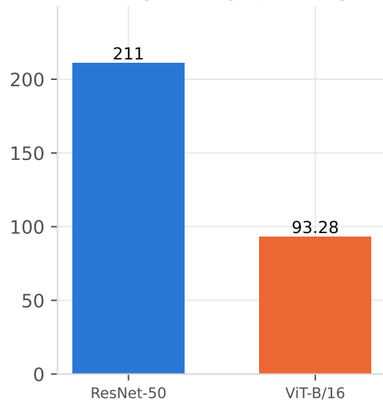
training throughput (img/s)
