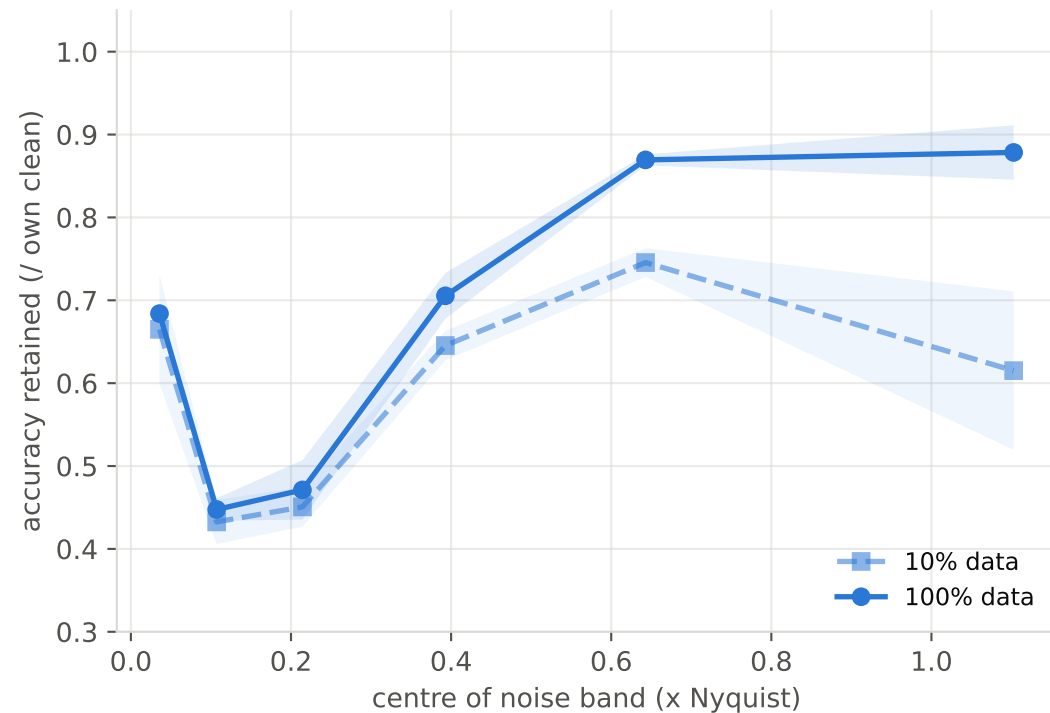
ResNet-50 (CNN)
