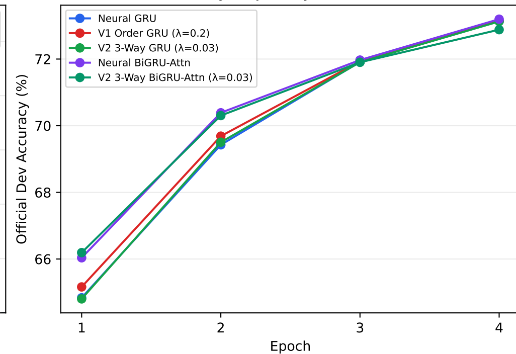
Dev Accuracy Trajectory (Mean of 3 Seeds)
