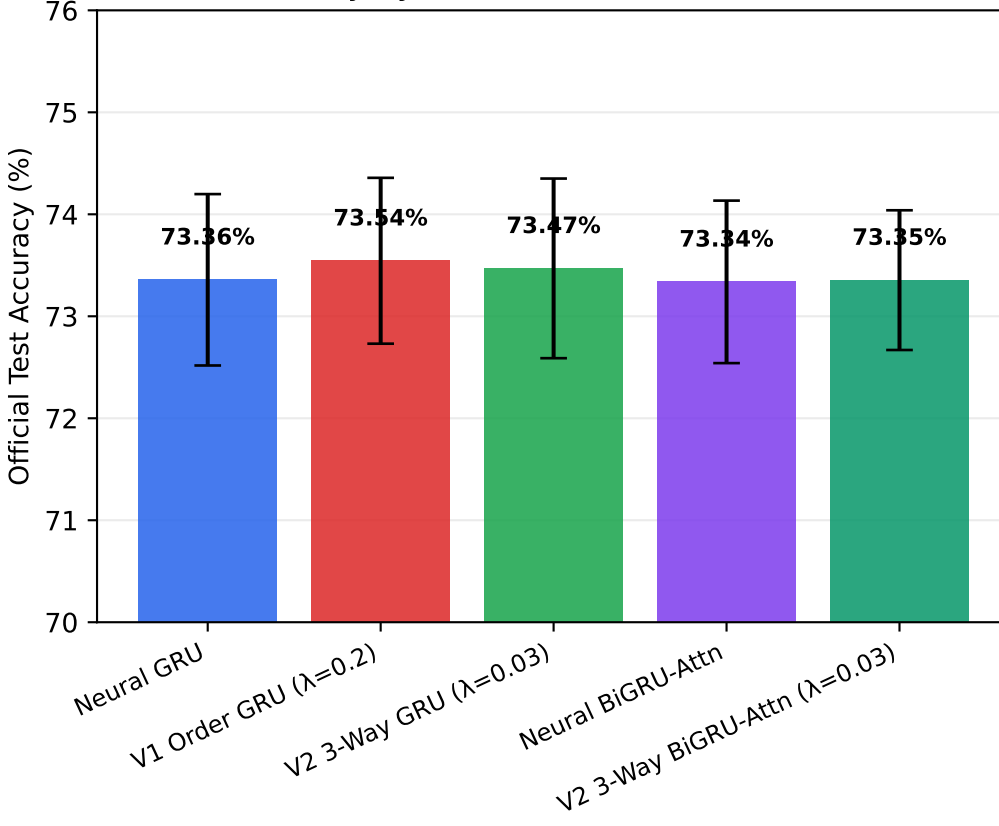
Test Accuracy by Model Arm (Mean \pm SD, 3 Seeds)
