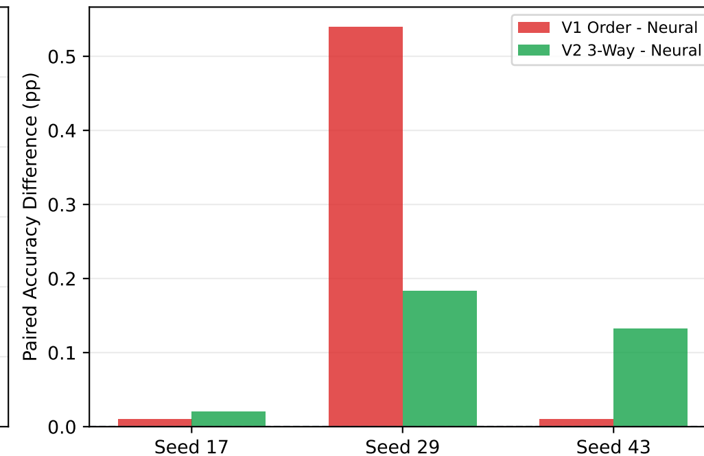
Track A (GRU): Paired Difference vs Neural Baseline
