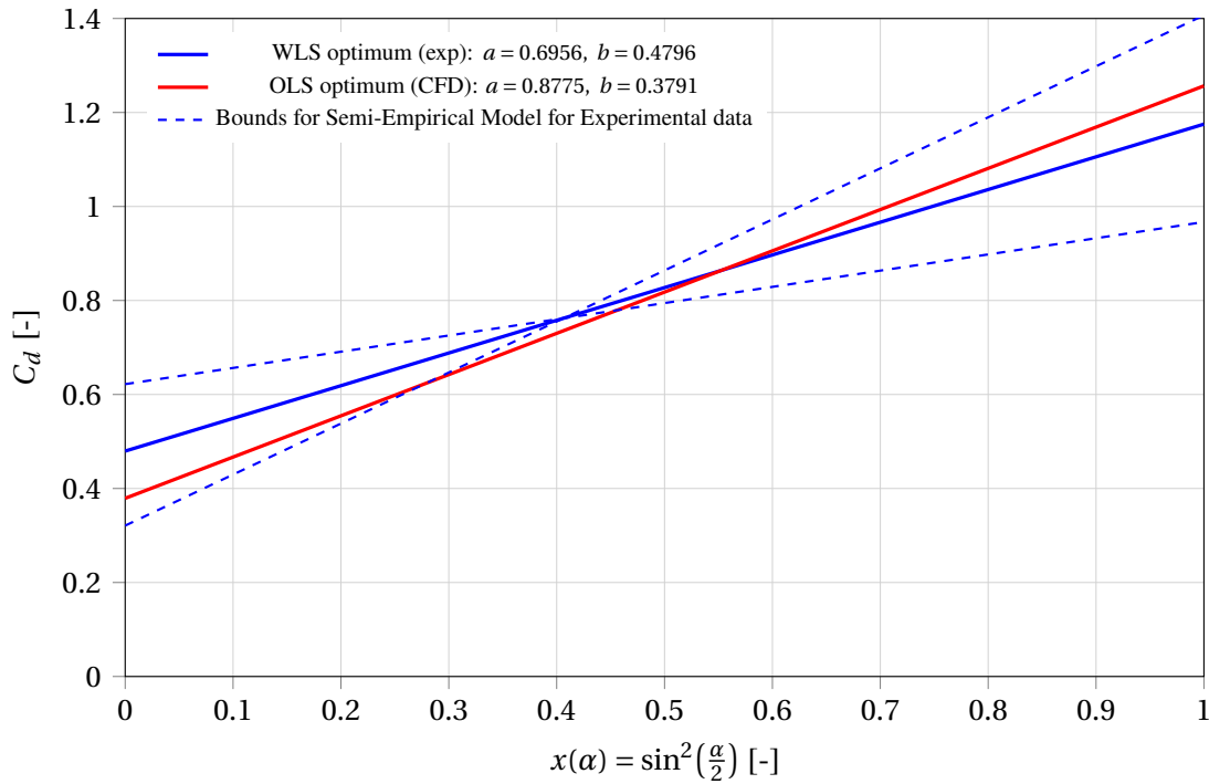
Figure 6.7: Comparison of semi-empirical models in the space x(\alpha) = \sin^2(\frac{\alpha}{2}) : Experimental WLS fit and pivot envelope and CFD OLS fit.
