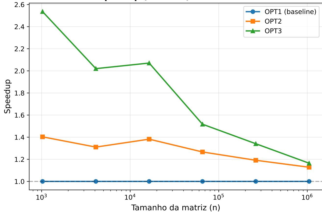
Speedup (vs OPT1) - Bandas=27
