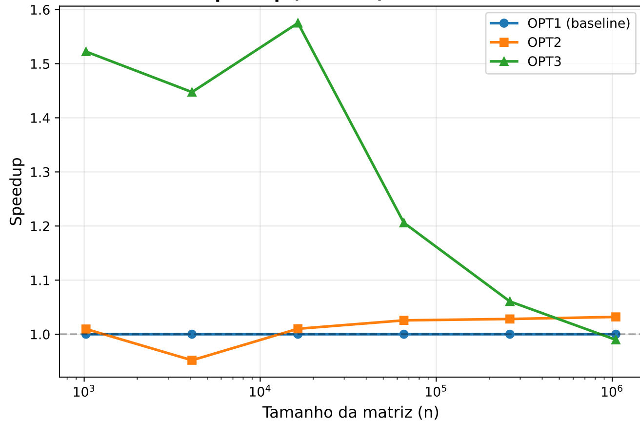
Speedup (vs OPT1) - Bandas=7
