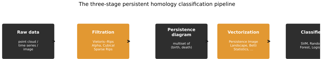
Figure 1.1: The three-stage persistent homology classification pipeline.
