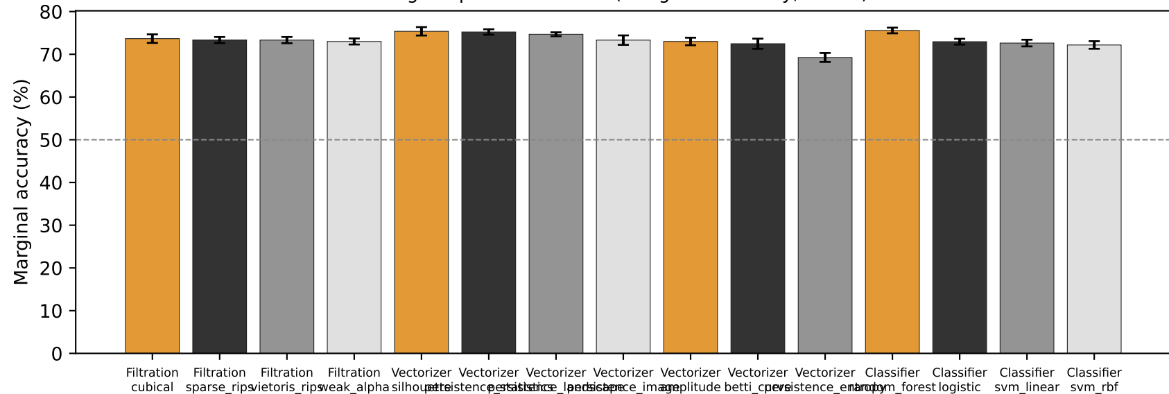
Stage impact on ECG200 (marginal accuracy, \pm 1 SE)
