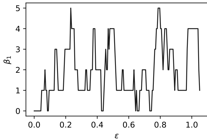
Betti curve
