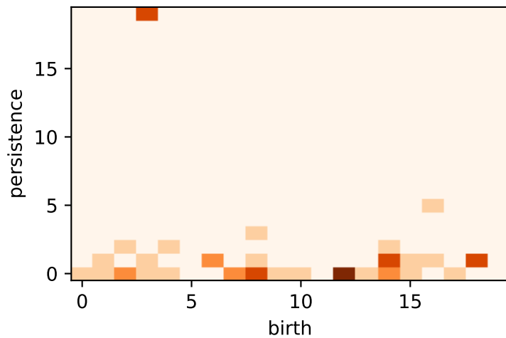
Persistence image
