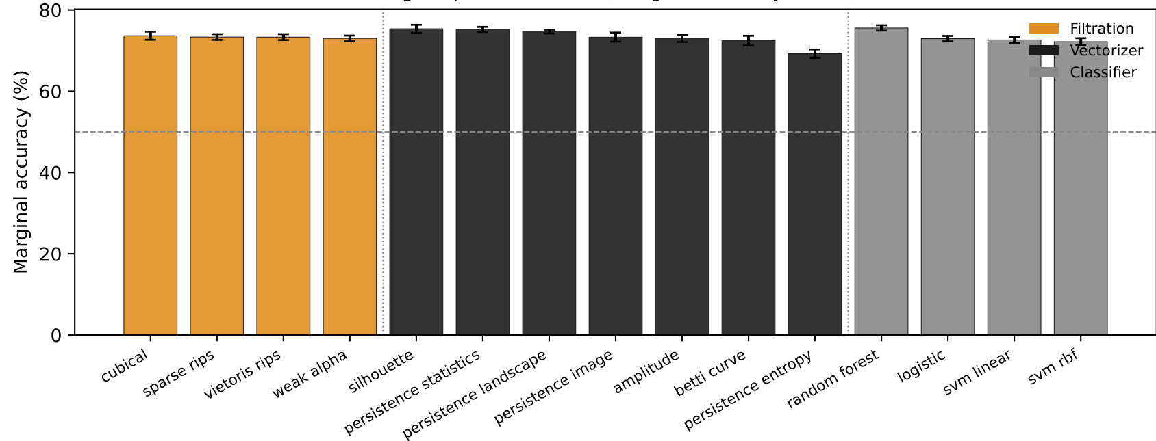
Stage impact on ECG200 (marginal accuracy, \pm 1 SE)
