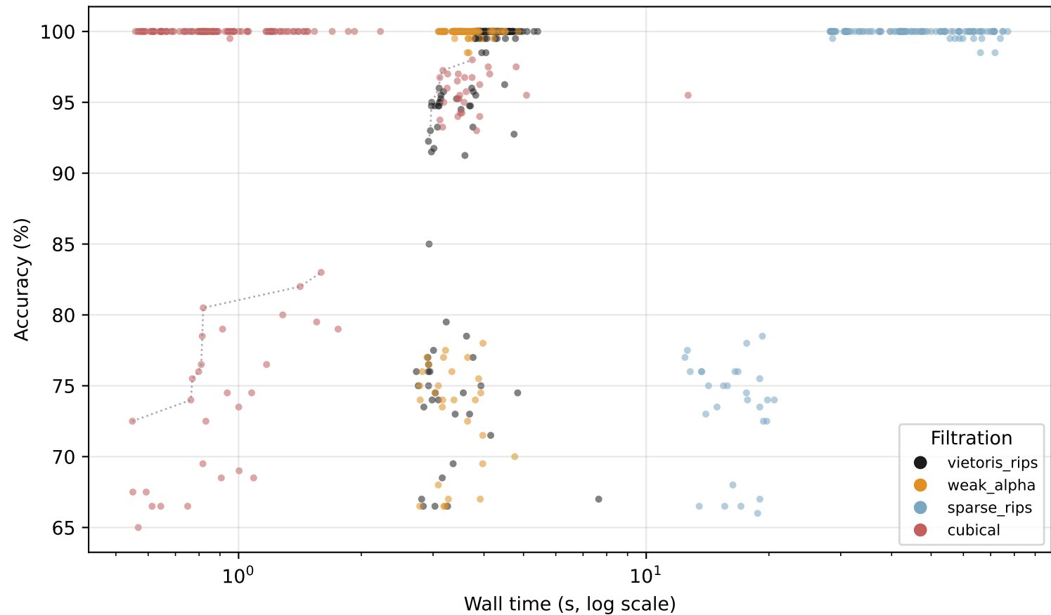
Runtime vs. accuracy across all 616 configurations
