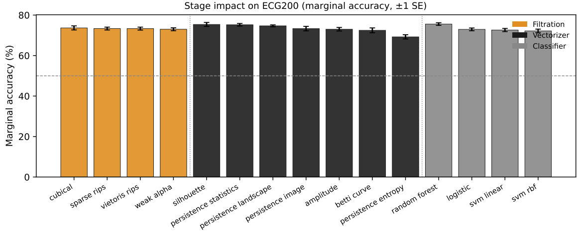
Figure 4.1: Stage impact on ECG200. Error bars show \pm 1 SE.
