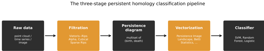
Figure 1.1: The three-stage persistent homology classification pipeline.
