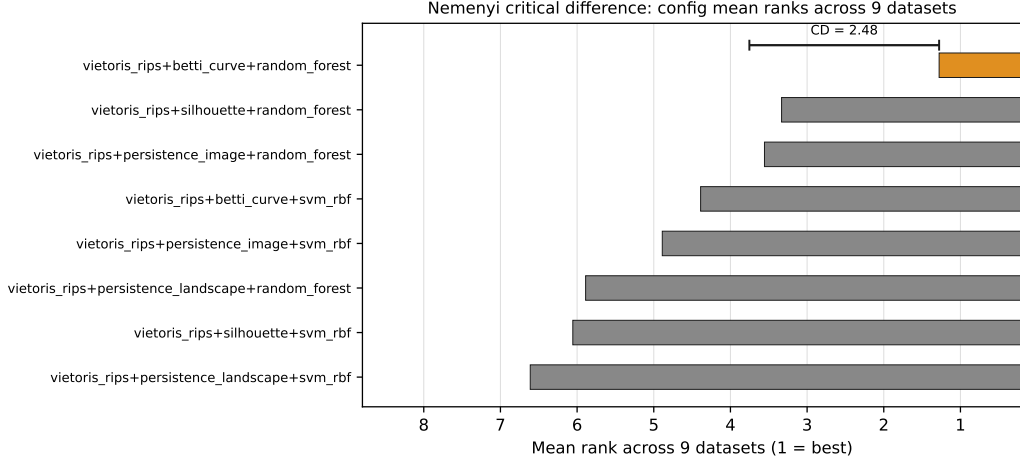
Figure 4.4: Nemenyi critical-difference diagram: configuration mean ranks across the 9-dataset panel (1 = best). The bracket marks the CD at \alpha=0.05 ; configurations outside it are significantly worse than the best.
