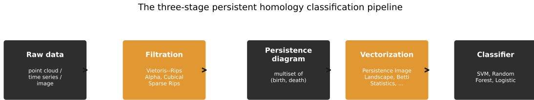
Figure 1.1: The three-stage persistent homology classification pipeline.
